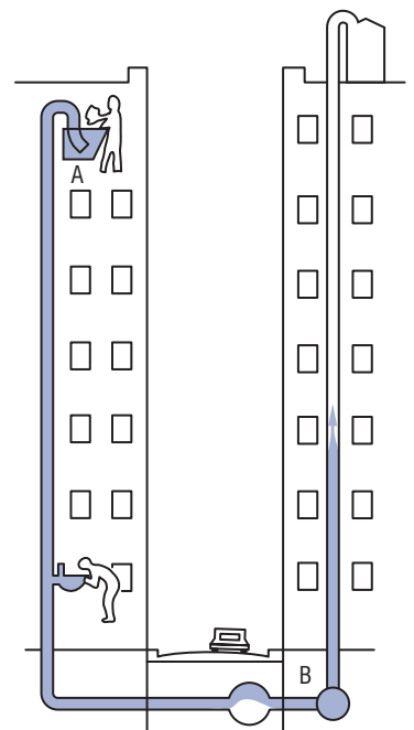
FIGURE 45. Backsiphonage (Case 2).
