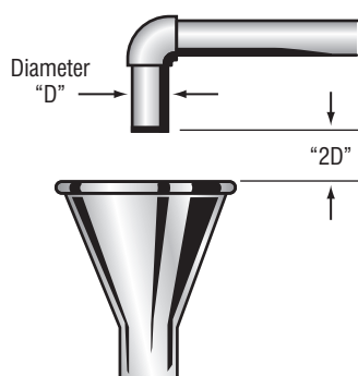
FIGURE 12. Air gap.
